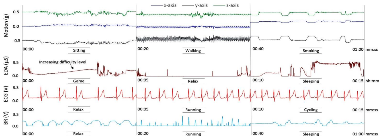
Figure 4: Motion, EDA, ECG & BR time domain signals under different situations
